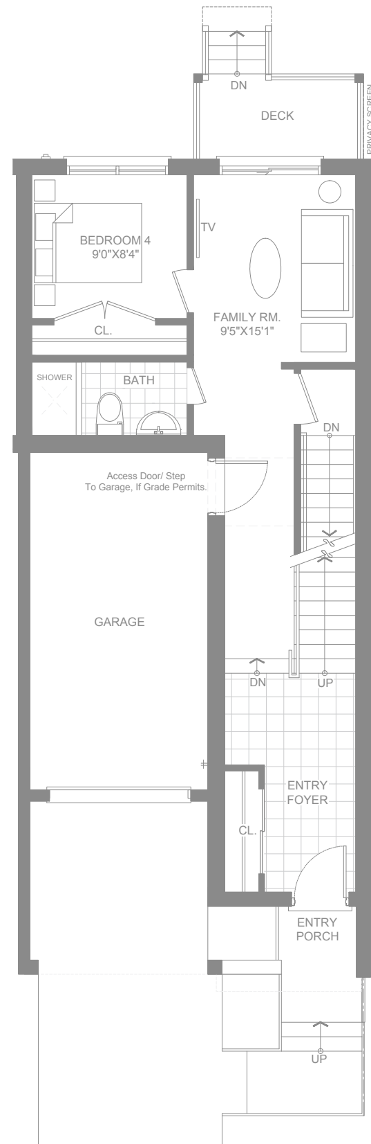
GROUND FLOOR - CG1
