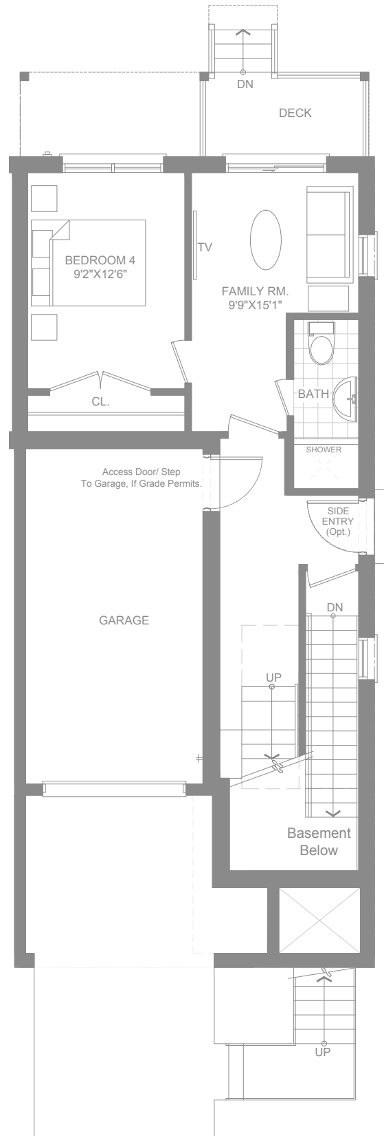
GROUND FLOOR - BG1E
