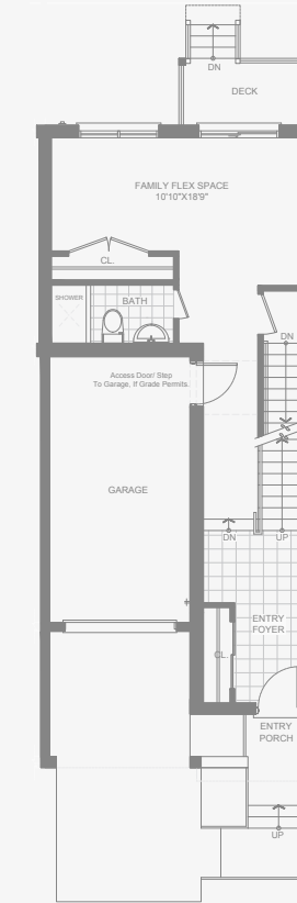
GROUND FLOOR CG2
