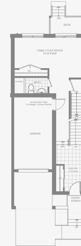
GROUND FLOOR CG2E
